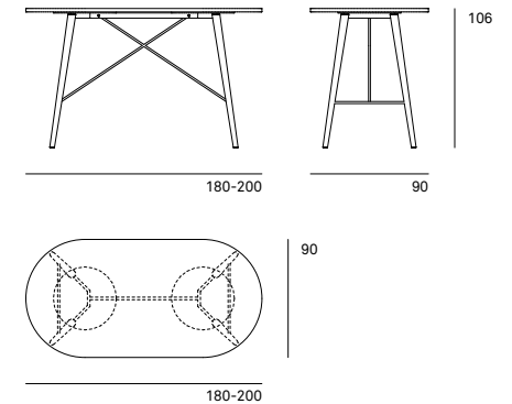
222/91 Oval
